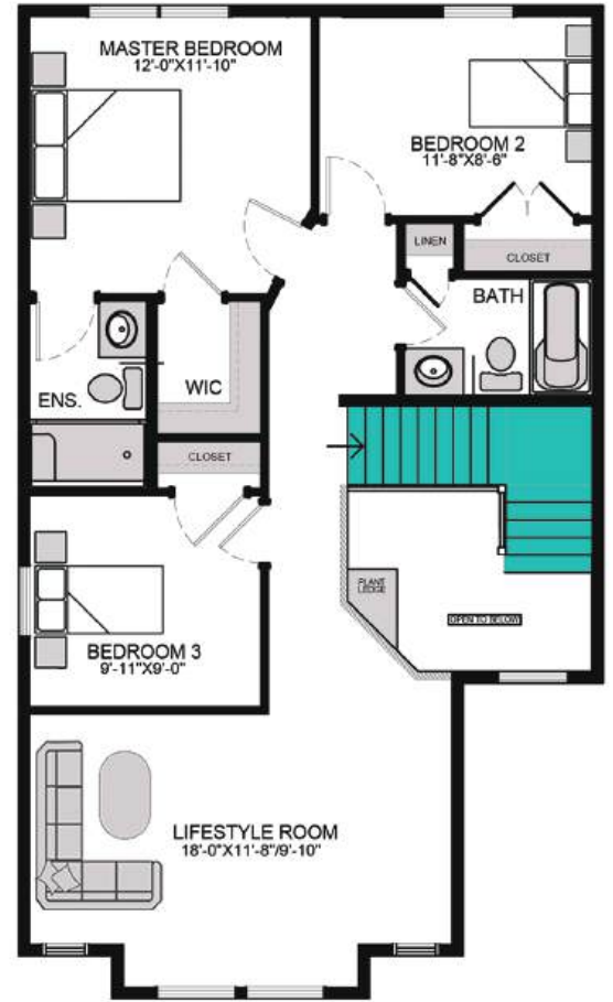
SECOND FLOOR: 877 sq ft
